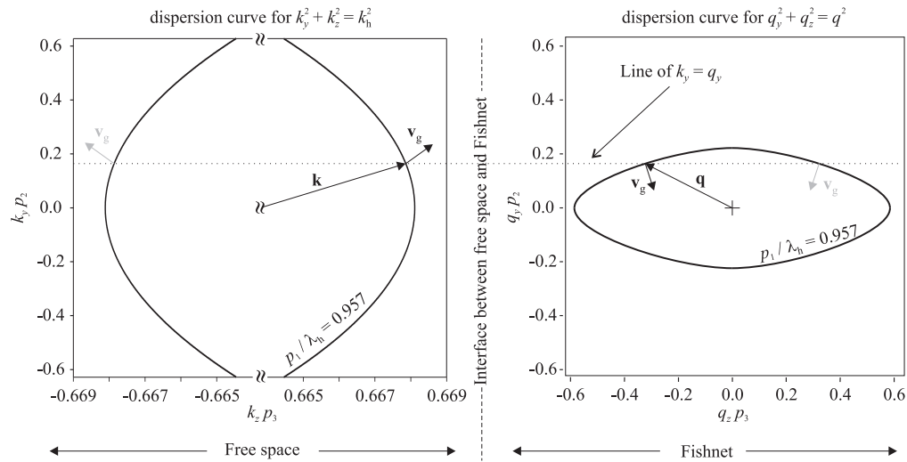
Fig. 5. Graphical representation of TM polarized plane wave refraction on the planar boundary between free space and fishnet. Group velocity is signed as \mathbf{v}_g , with black arrows corresponding to the waves propagating along the z -axis and gray arrows corresponding to the waves in the opposite direction. Note that the phase velocity in z direction v_{fz} = \omega/k_z or v_{fz} = \omega/q_z is positive for the wave on the left panel and negative for the right panel.
